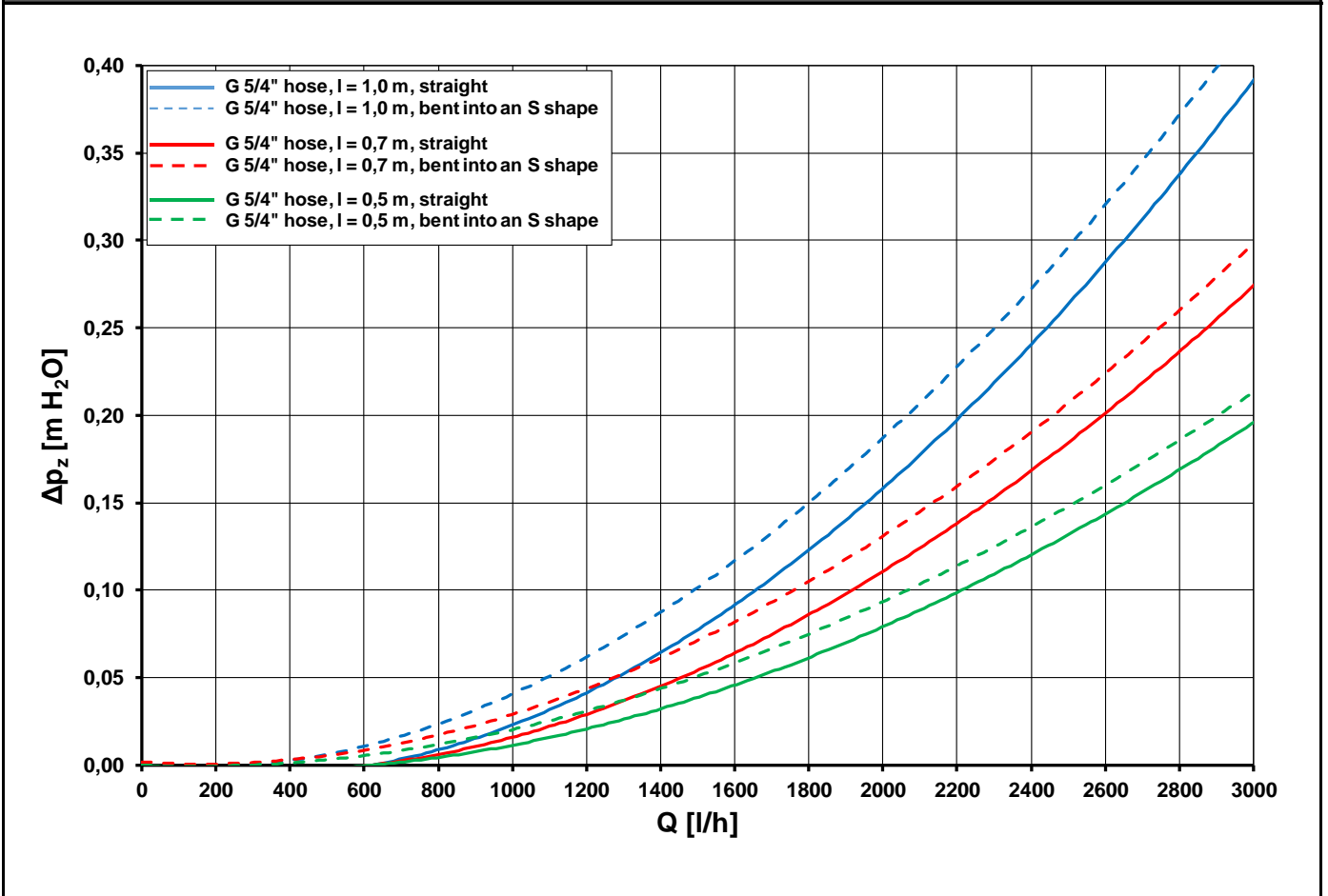
Pressure drop graph for a G 5/4" hose
